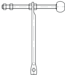
Adjustable protective horn
