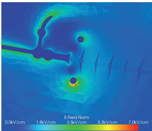
Example for a computation of fields (Lapp Insulators)
