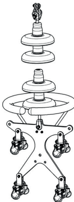
Arcing rings for UHV lines
