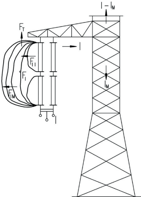
Cascaded power arcs are united to one overall power arc
