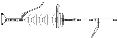
Tension string with cap and pin type insulators with long arcing devices
