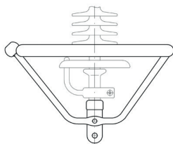
Corona ring and arcing device
