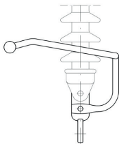
Lower one-way arcing ring with a long rod insulator
