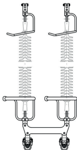
Arrangement of arcing devices in case of a double suspension string
