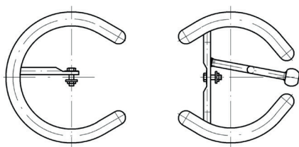
Combination of arcing rings for double suspension strings
