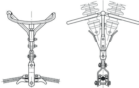
Arcing rings for rigid V-strings
